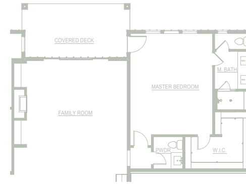
Main Floor Deck Extension Option
