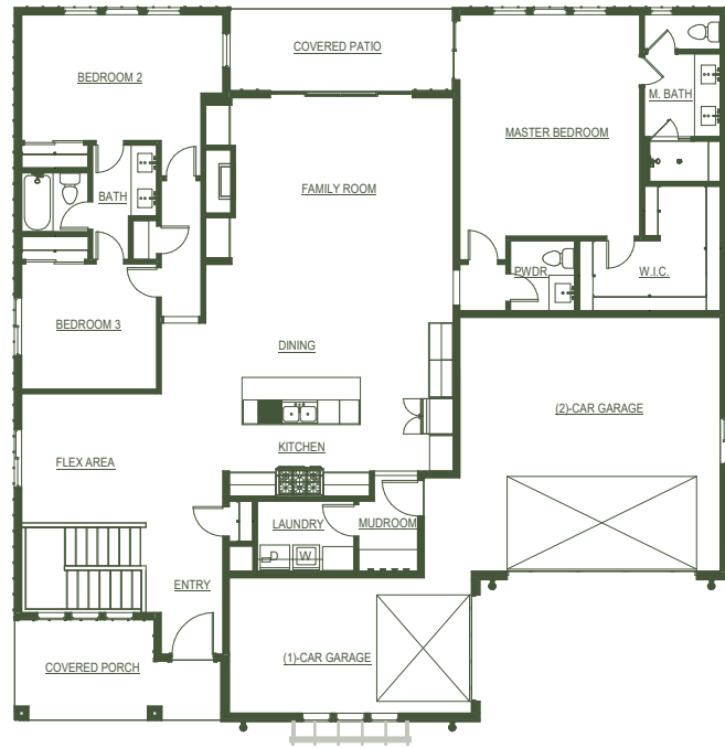
Main Floor 2,310 SF
